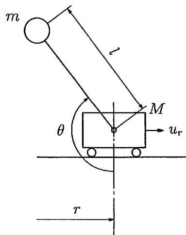
Fig.1 A cart and pendulum system
