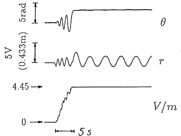
Fig.3 The results of experiments
